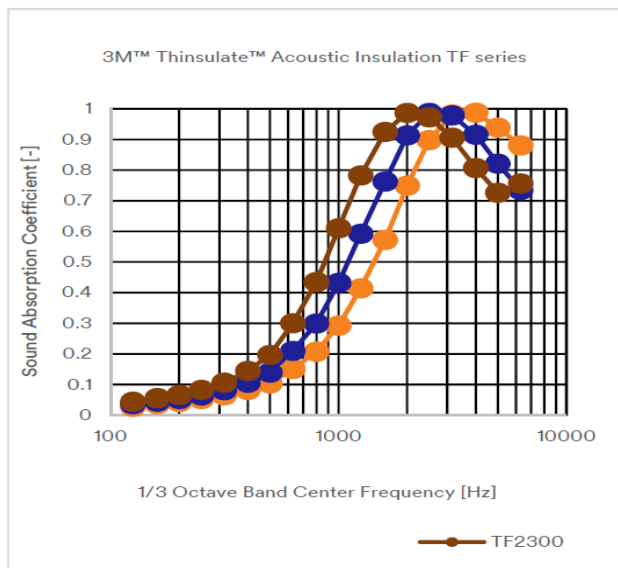
Typical Normal Incident Absorption Coefficient per ASTM E-1050
