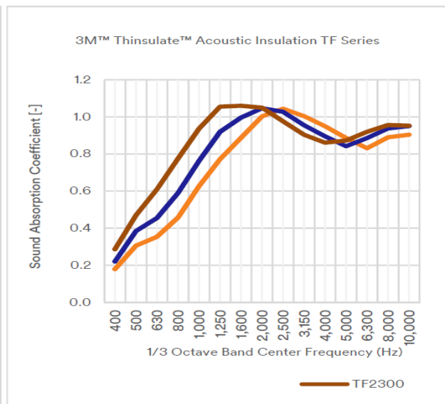
Typical Random Incident Absorption Coefficient per SAE J2883
